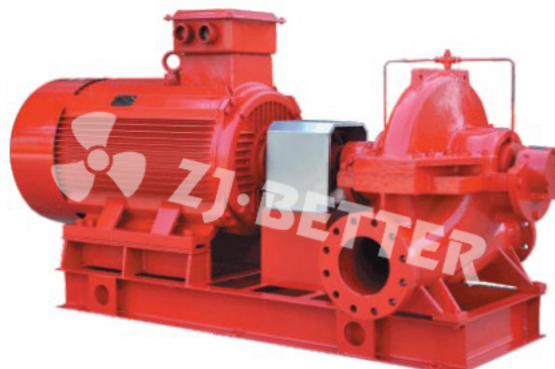
UL Electric Split Case Pump
