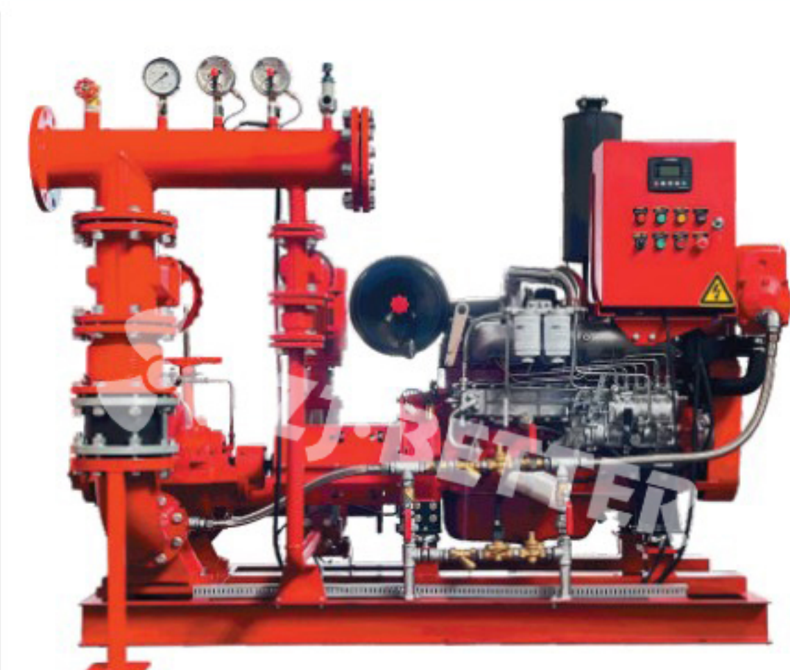
Split Case Fire Pump Set
